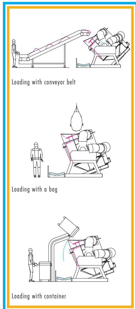
Front view loading - the cage tilts up to 70° upwards
